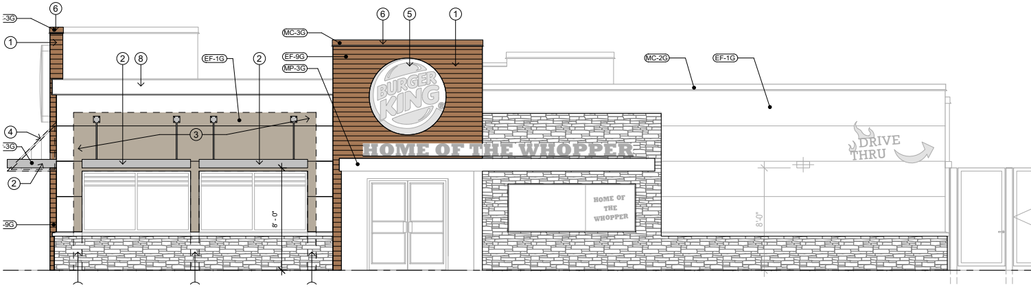
2 WEST ELEVATION 1/4" = 1'-0"
