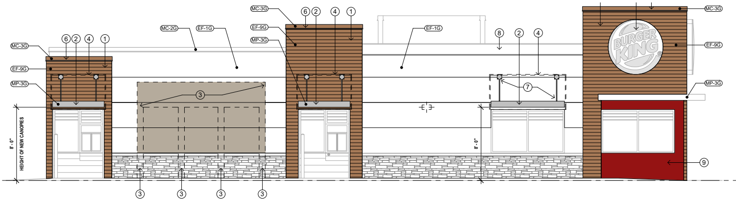
2 WEST ELEVATION 1/4" = 1'-0"
